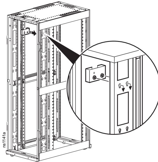
Wire Management Bracket (6)
